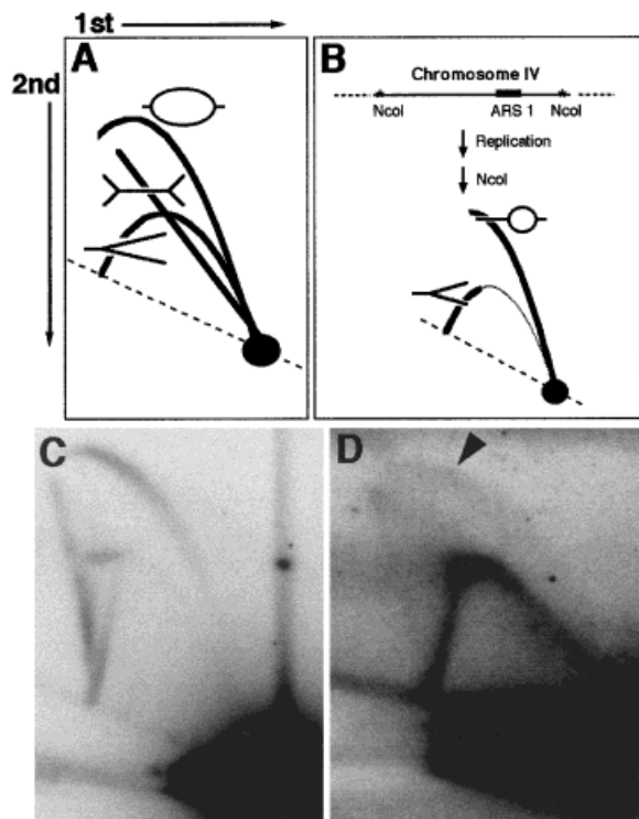
Fig. 6. Analysis of the sites of initiation in the vicinity of the ARS1 chromosomal origin. A: Schematic diagram illustrating the general principle of the neutral-neutral 2D-gel assay, showing the theoretical migration patterns of replication bubbles, double Y, and replication fork structures. B: Schematic diagram illustrating the principle of the 2D-gel assay, as it applies to analysis of the ARS1 origin. After digestion of genomic DNA containing replication intermediates with NcoI , initiation uniquely within the ARS1 origin should reveal a typical replication bubble structure, collapsing into a fork arc within molecules in which the replication forks have traveled beyond the NcoI sites. C: Genomic DNA was isolated from asynchronously growing cultures of JW-1 cells, digested with NcoI , subjected to 2D-gel electrophoresis, and hybridized with a 5-kb NcoI fragment encompassing ARS1. D: Intact G1-phase JW-1 nuclei were incubated for 60 min in Xenopus egg extract supplemented with 3 \mu\text{g/ml} aphidicolin for 90 min. Genomic DNA was purified, digested with NcoI , and subjected to 2D-gel analysis as in (C). The arrowhead indicates the position of a faint but reproducible bubble arc.
