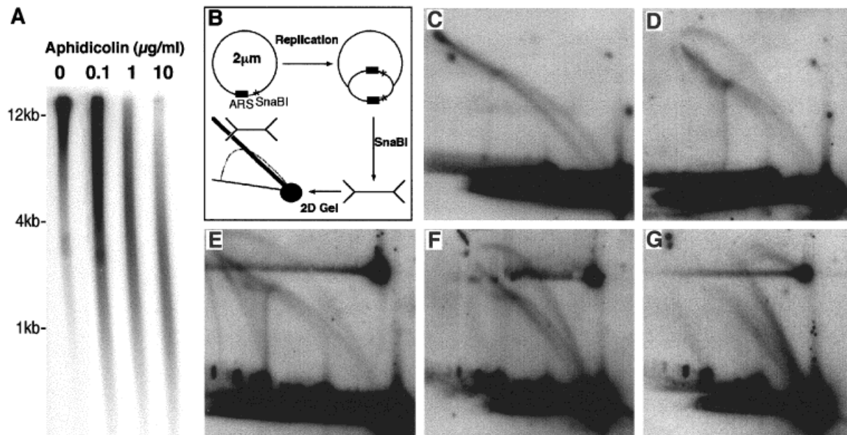
Fig. 5. Analysis of the sites of initiation within the 2- \mu m plasmid. A: Intact G1-phase JW-1 nuclei were incubated in Xenopus egg extract containing [ \alpha - ^{32} P] dATP and the indicated concentrations of aphidicolin for 90 min. Isolated DNA was subjected to alkaline agarose gel electrophoresis. Molecular weight markers are indicated on the left of the gel. B: Schematic diagram illustrating the principle of the neutral-neutral 2D-gel assay as it applies to analysis of the 2- \mu m circle. Replicated DNA molecules are separated in the first dimension by size and in the second dimension by shape. SnaBI digestion of replication intermediates within plasmids that initiate at the unique 2- \mu m origin produces a double-Y structure that migrates as a
