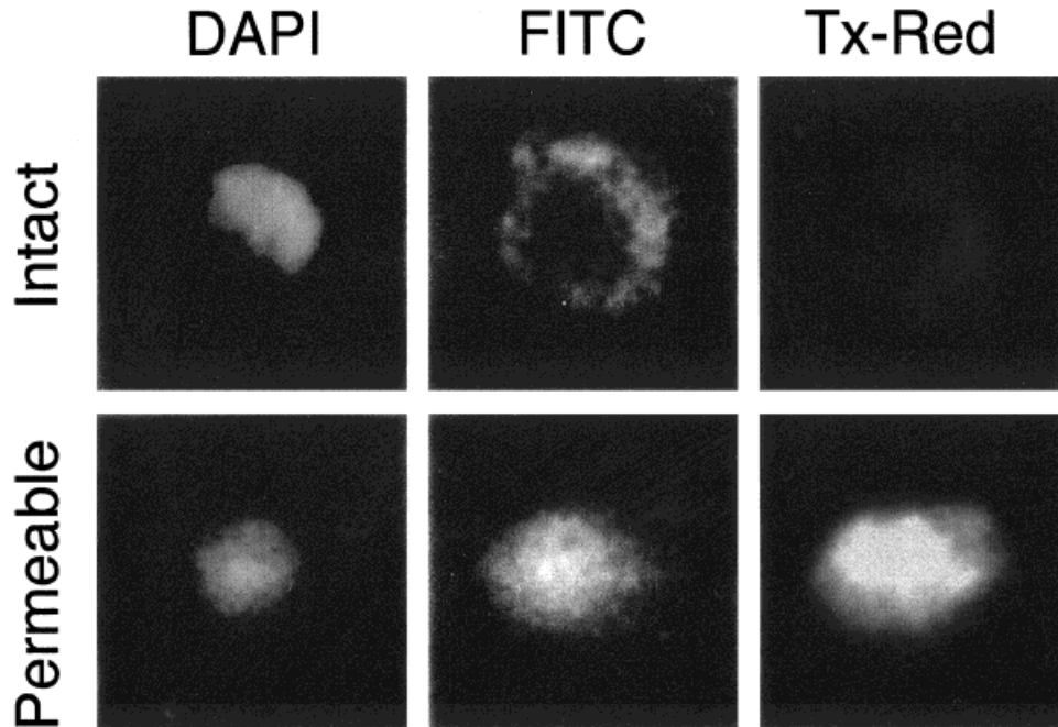
Fig. 1. Assay for intact versus permeabilized nuclei. Intact nuclei were prepared and stained simultaneously with an antibody against a nuclear pore epitope present on the outer surface of the nucleus (MAb414) and an anti-histone H4 antibody, as described in Materials and Methods. DNA was counterstained with DAPI. Aliquots of these nuclei were permeabilized by incubation with 0.02% Triton X-100 on ice for 5 min. Intact nuclei are decorated on the surface with MAb414 but are
