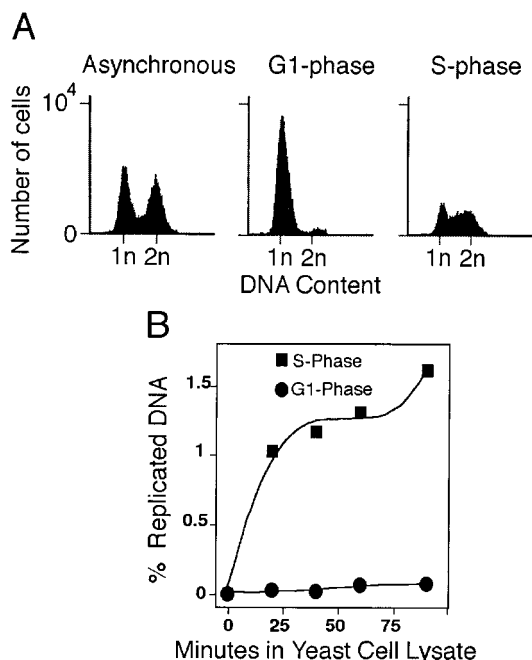
Fig. 2. Evaluation of cell synchrony. A: JW-1 cells were collected either during asynchronous growth, after \alpha -factor arrest for 3 h (G1-phase), or after release from \alpha -factor arrest for 30 min (S-phase) and analyzed by flow cytometry. B: G1-phase and S-phase nuclei were incubated with a replication cocktail containing [ \alpha - ^{32} P] dATP and the total counts per minute were incorporated into high-molecular-weight DNA determined by acid precipitation. Parallel reactions with the same nuclear preparations were incubated in the presence of aphidicolin, and the counts per minute incorporated in the presence of aphidicolin were subtracted from that detected in the absence of aphidicolin to reveal the aphidicolin-sensitive counts per minute incorporated, a measure of nuclear replicative DNA synthesis. The percent of total input DNA replicated during the in vitro labeling period was then calculated and plotted as percent replicated DNA.
