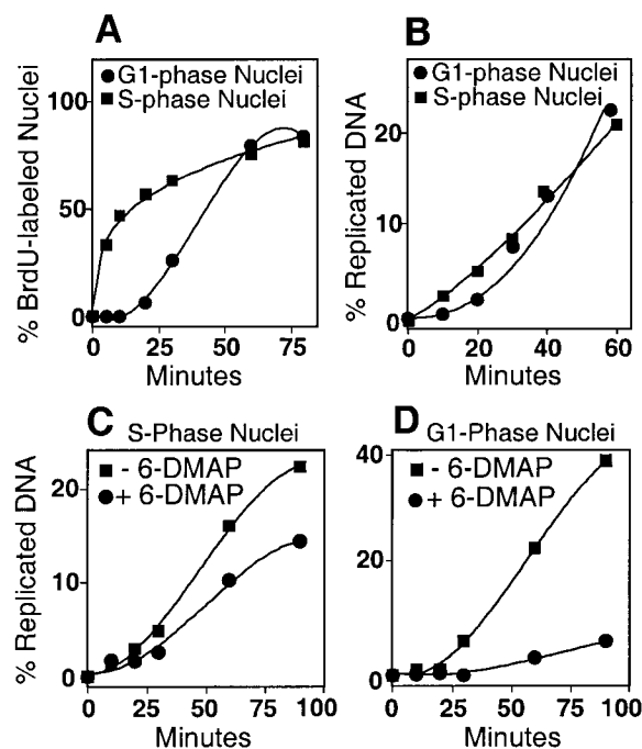
Fig. 4. Properties of DNA synthesis with G1-phase versus S-phase nuclei in Xenopus egg extract. A,B: Intact JW-1 G1-phase and S-phase nuclei were introduced into Xenopus egg extract containing BrdUTP (A) or [ \alpha - 32 P] dATP (B). At the indicated time, aliquots from these reactions were removed, and either the percentage of nuclei that incorporated BrdU (A) or the percentage of genomic DNA replicated (B) was determined as described in Materials and Methods. In (B), the counts per minute (cpm) incorporated in parallel reactions carried out in the presence of aphidicolin were subtracted from the cpm in the absence of aphidicolin and the percentage of total input DNA replicated was calculated from the total aphidicolin-sensitive cpm incorporated, as in Figure 1. C,D: Intact JW-1 S-phase (C) and G1-phase (D) nuclei were introduced into Xenopus egg extract containing [ \alpha - 32 P] dATP in the presence (circles) or absence (squares) of 6-DMAP. The percentage of input DNA replicated was calculated from the aphidicolin-sensitive cpm incorporated as in (B).
