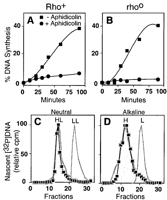
Fig. 3. DNA synthesis in Xenopus egg extract results from semiconservative DNA replication. A: Intact G1-phase JW-1 nuclei ( \rho^+ ) were incubated in a Xenopus egg extract in the presence (circles) and absence (squares) of aphidicolin. The amount of DNA synthesized at each time point was determined by acid precipitation and plotted as a percent of input DNA. B: Intact G1-phase nuclei from an isogenic derivative of JW-1 lacking mitochondria ( \rho^0 ) were incubated in a Xenopus egg extract and the percent DNA synthesis was determined as in (A). C: \rho^0 -G1-phase nuclei were incubated in Xenopus egg extract supplemented with [ \alpha - ^{32} P] dATP and BrdUTP. Total genomic DNA was isolated and centrifuged to equilibrium in a neutral \text{Cs}_2\text{SO}_4 gradient, and the counts per minute (cpm) per fraction (squares) collected from the bottom of the tube was determined. The positions of unifilarly BrdU substituted marker- \text{C}^{14} -DNA (HL) and unsubstituted marker- \text{C}^{14} -DNA (LL), analyzed in parallel gradients, are indicated as solid gray lines. D: Neutral density gradient fractions indicated by the shaded region in (C) were pooled and centrifuged to equilibrium in an alkaline \text{Cs}_2\text{SO}_4 gradient and the cpm per fraction was determined as in (C). The positions of BrdU substituted marker- \text{C}^{14} -DNA (H) and unsubstituted marker- \text{C}^{14} -DNA (L), analyzed in parallel gradients, are indicated with a solid gray line as in (D).
